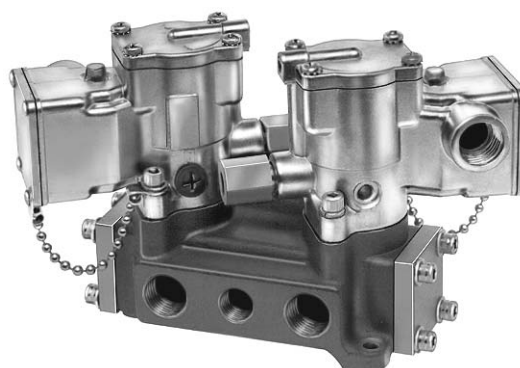
Double Solenoid
