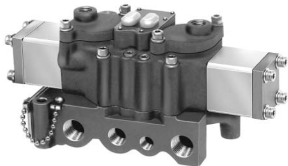
3/8" Basic, Nominal Cv = 4.8
