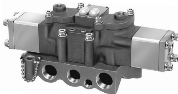
1/2" Basic, Nominal Cv = 5.0
