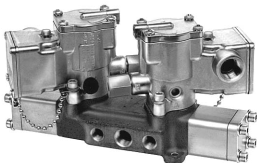
1/4" Basic, Nominal Cv = 1.7
