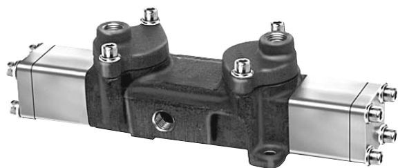
1/4" Basic, Nominal Cv = 1.7
